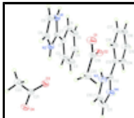
Fig. 1. The structure of (I), showing the atomic numbering scheme. Displacement ellipsoids are drawn at the 30% probability level.
